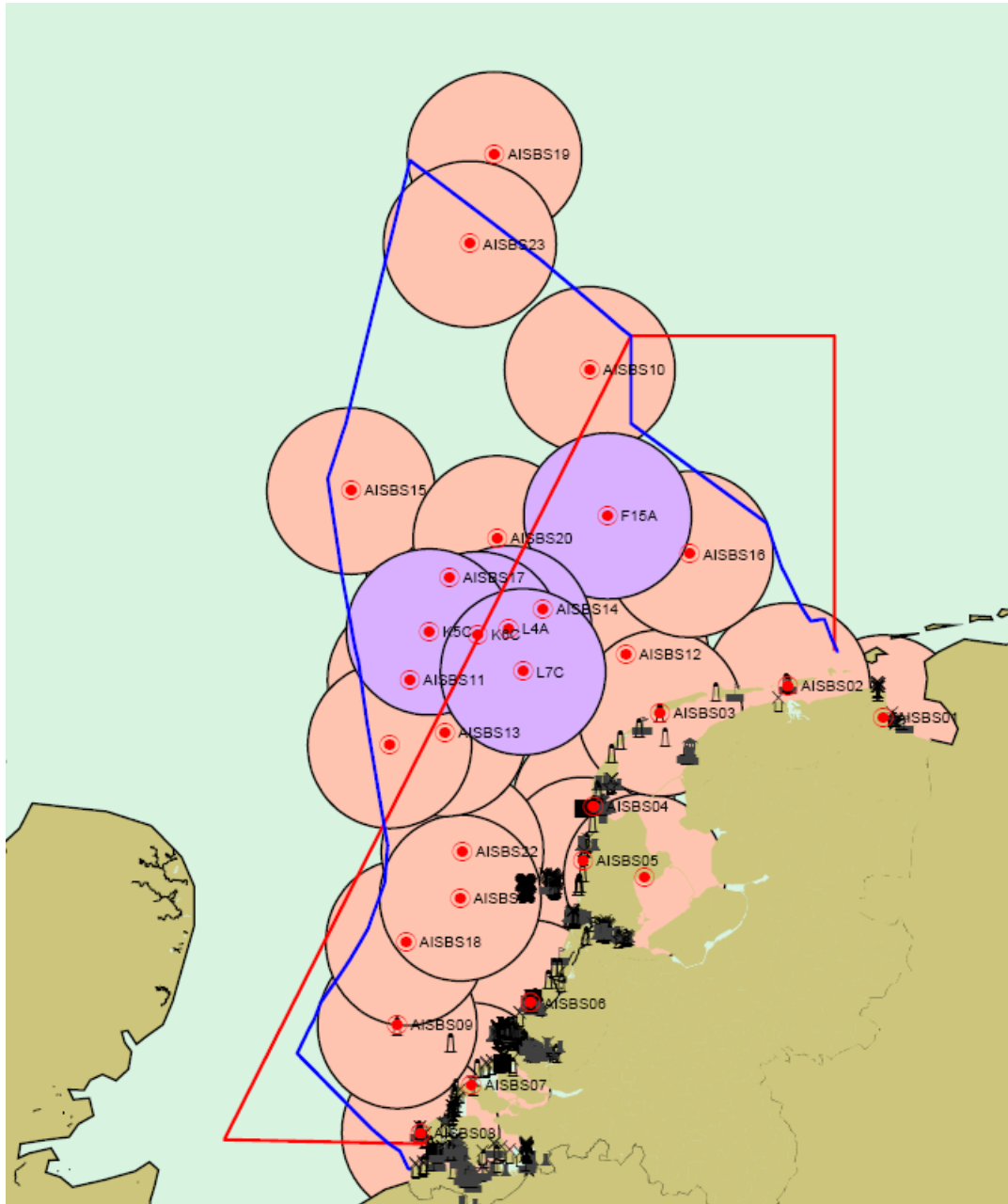
Figure 5-1 AIS base stations delivering data to the Netherlands Coastguard, the blue line illustrates the NCS, the circles indicate the reach of the base stations, the purple circles indicate the newest base stations
